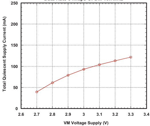
RMPA2550 Total Quiescent Bias Current Vs. VM Voltage 2.45 GHz VM, VC=3.3V T=25C Data Rate 54Mbps OFDM 16.7MHz
