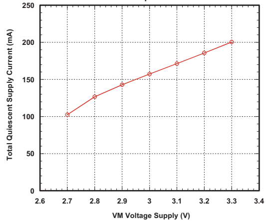
RMPA2550 Total Quiescent Bias Current Vs. VM Voltage 5.45 GHz VM, VC=3.3V T=25C Data Rate 54Mbps OFDM 16.7MHz
